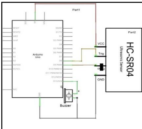
Fig. 2. Schematic diagram of SWCMAS
